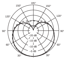
MX150/C Polar Pattern
